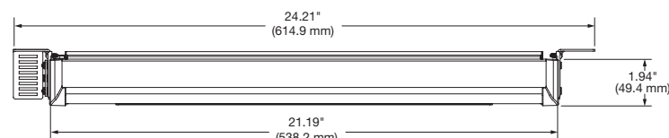
CCD 320 Front View
