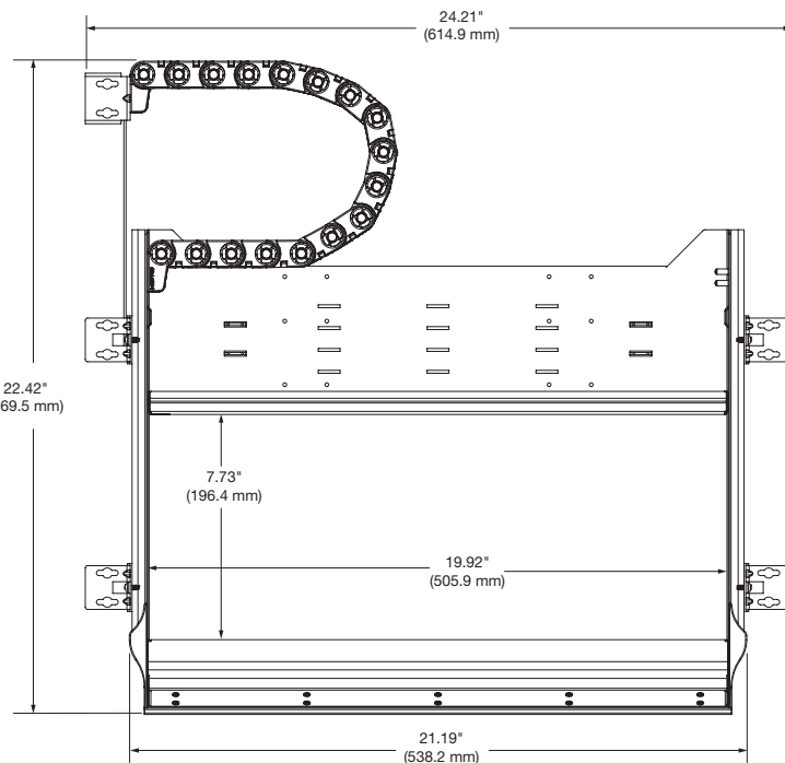
CCD 320 Top View
