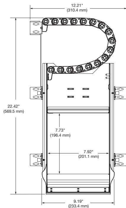
CCD 220 Top View
