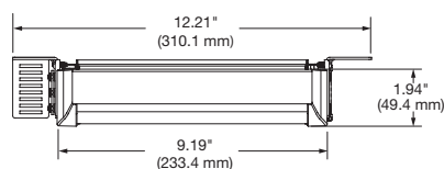
CCD 220 Front View
