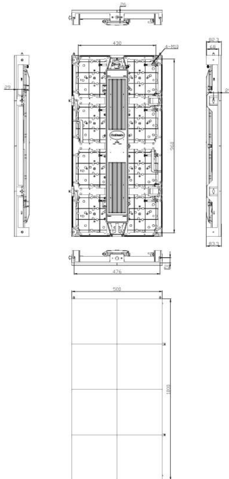
Fig1. Cabinet Dimension
