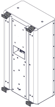
Domino-KF212 and integrated wall bracket
