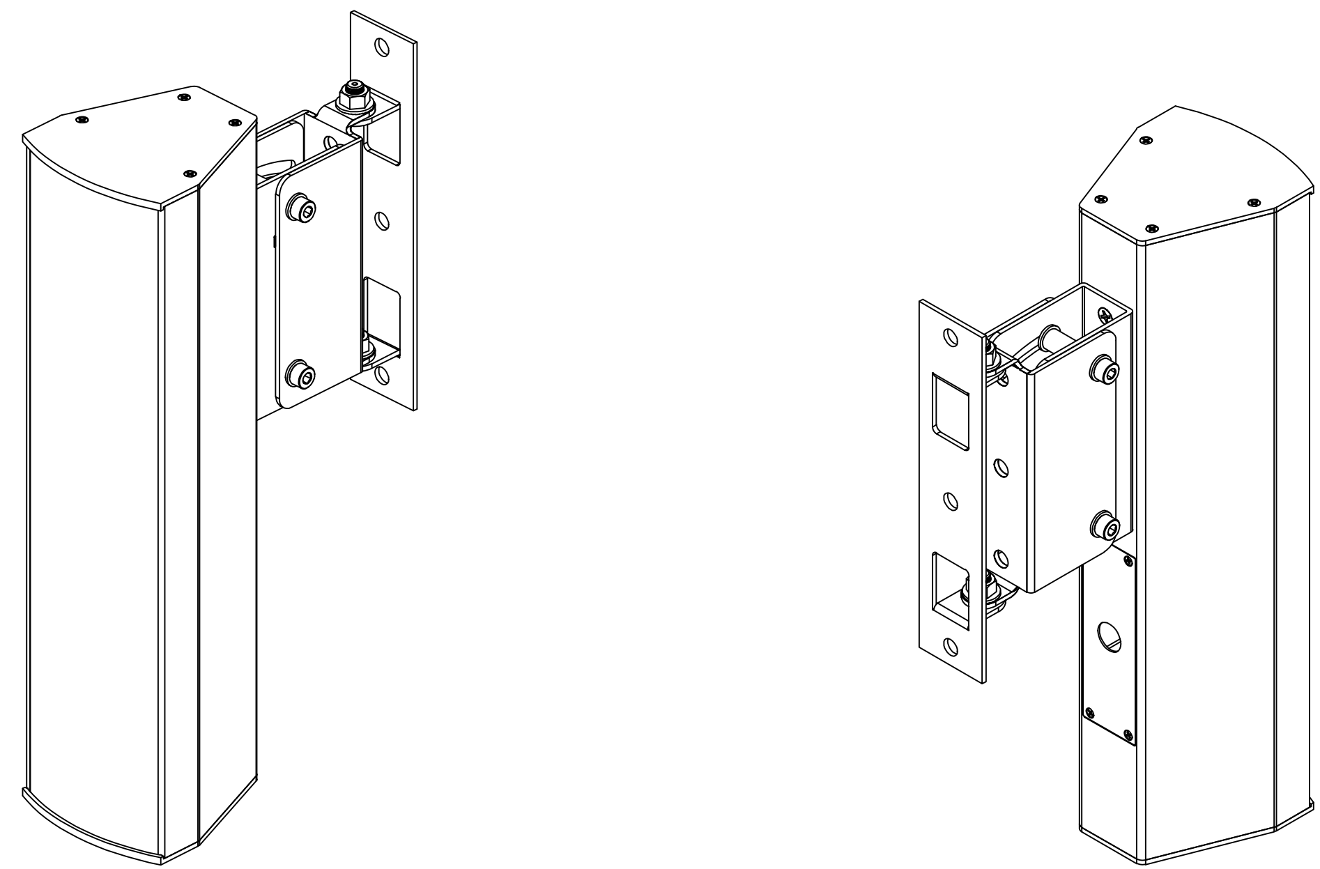
UBX4 WITH PAN & TILT BRACKET ASSEMBLY
