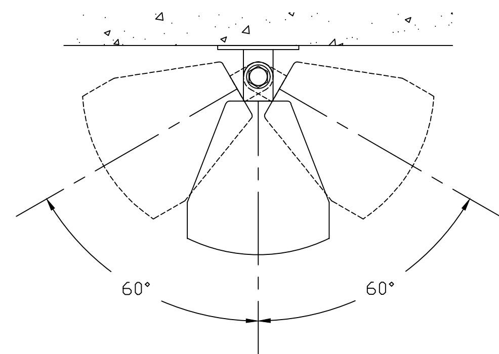
WALL MOUNT PANNING RANGE
