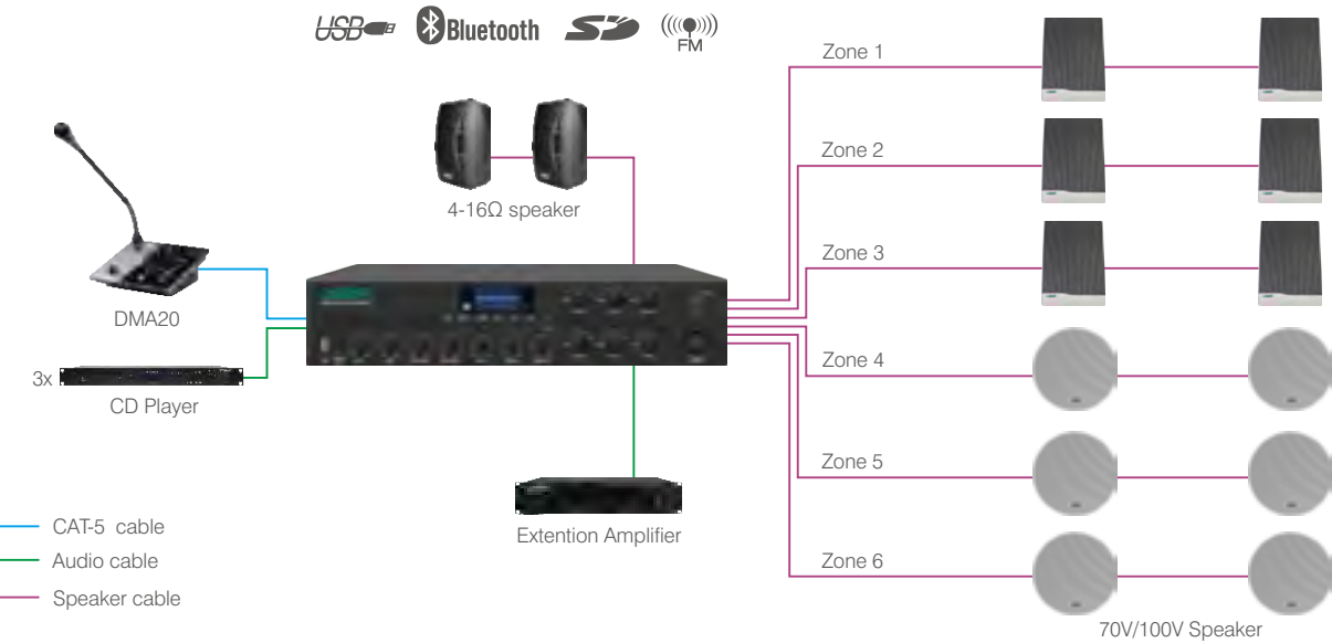
DC24V 4-16Ω & 70V/100V speaker outputs
