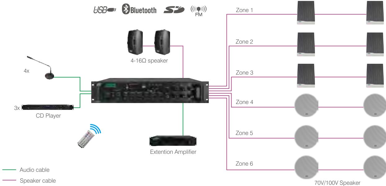
4 Mic and 3 Aux inputs
