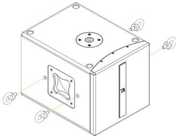
Thunder-KMT18P I suspending accessory
