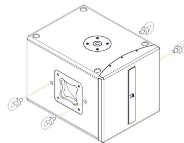
Thunder-KMT12P I suspending accessory
