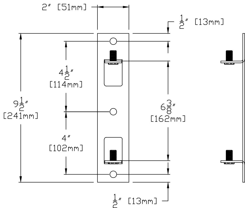
WALL BRACKET
