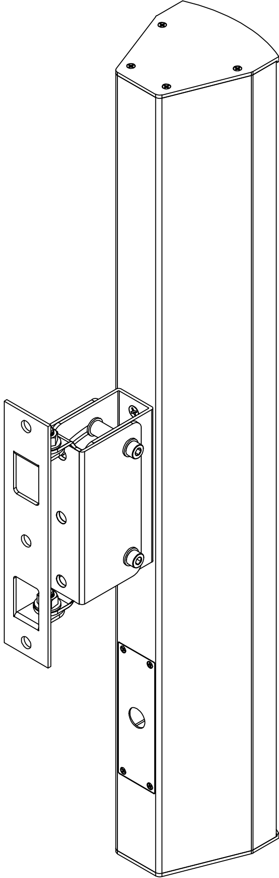
UBX8 WITH PAN & TILT BRACKET ASSEMBLY
