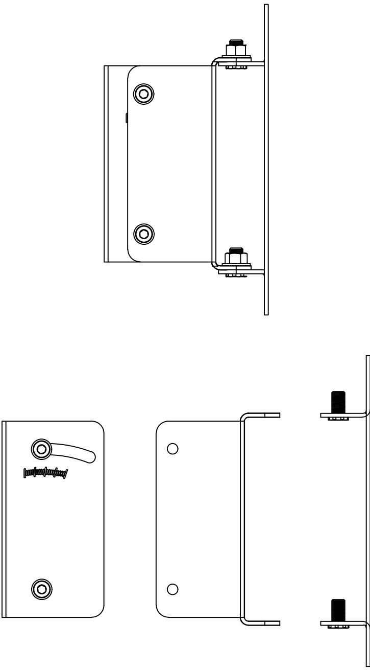
PAN & TILT BRACKET
